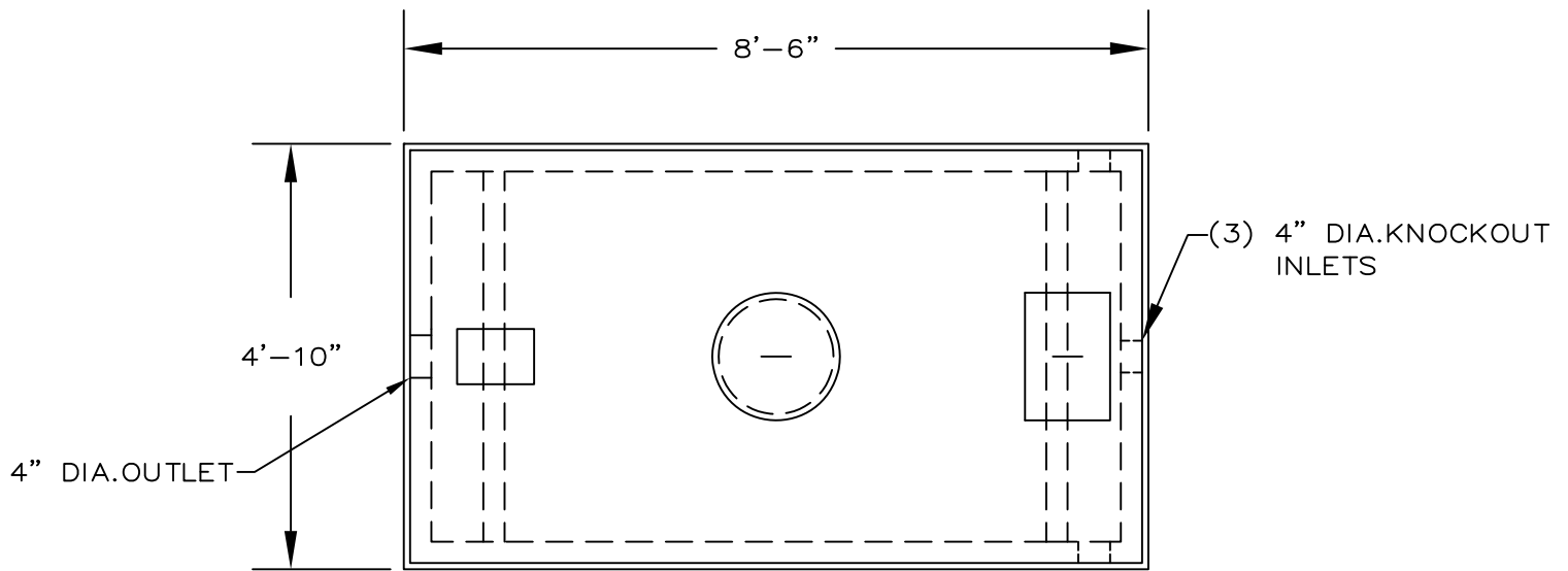
PLAN VIEW
