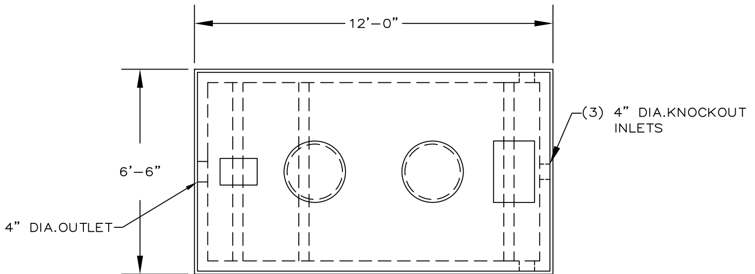
PLAN VIEW
