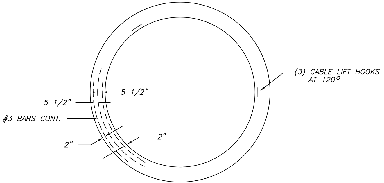
PLAN VIEW
